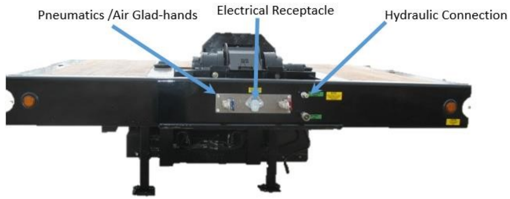
Front View of Trailer
