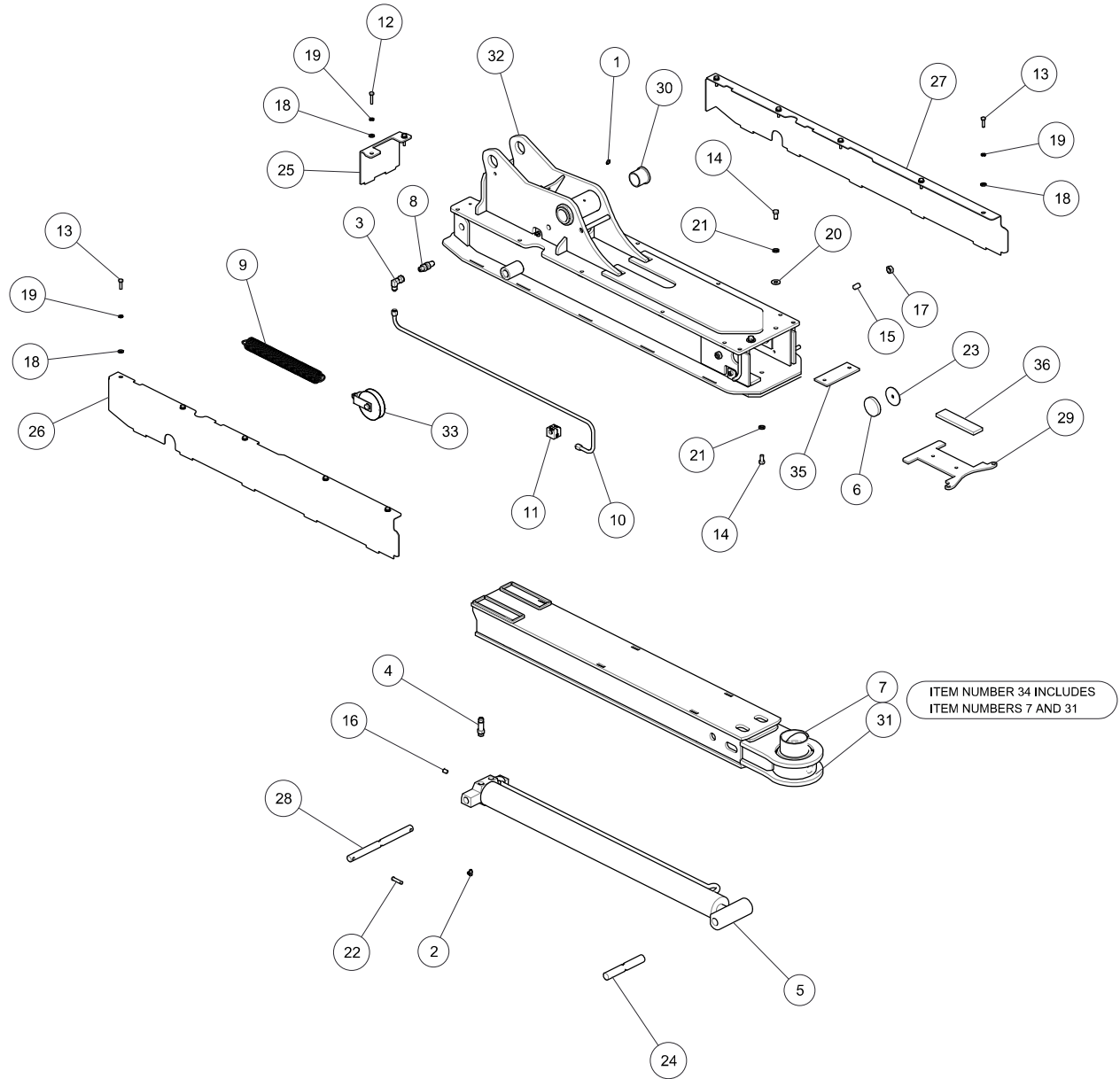
Figure 8. 812 Wheel Lift Figure
