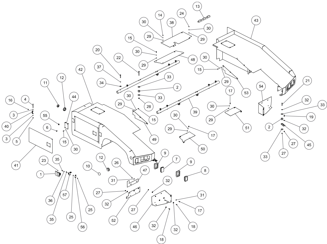
Figure 3. 812 Body Assembly Stainless
