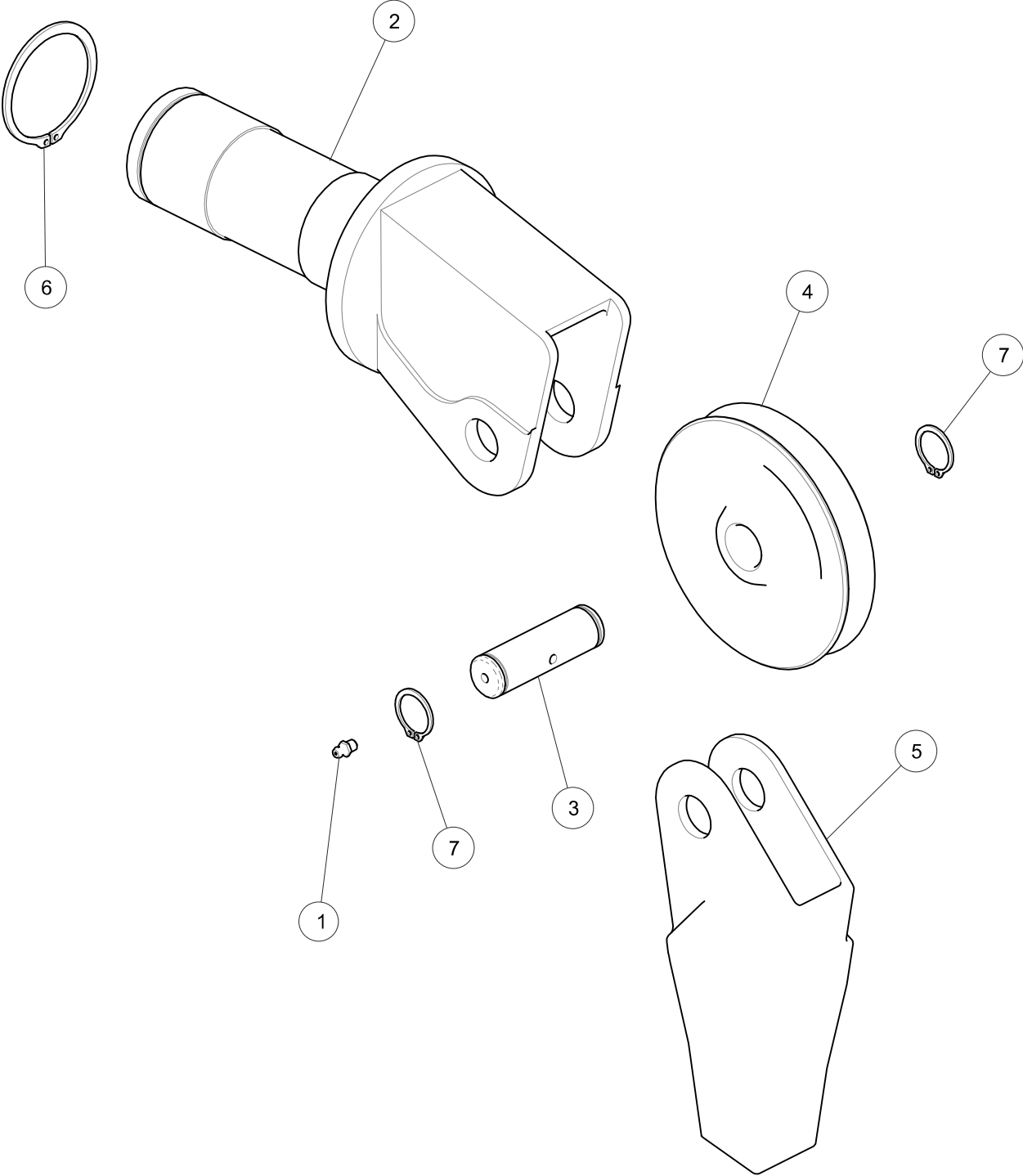
Figure 9. 812 Sheave Housing Assembly Figure
