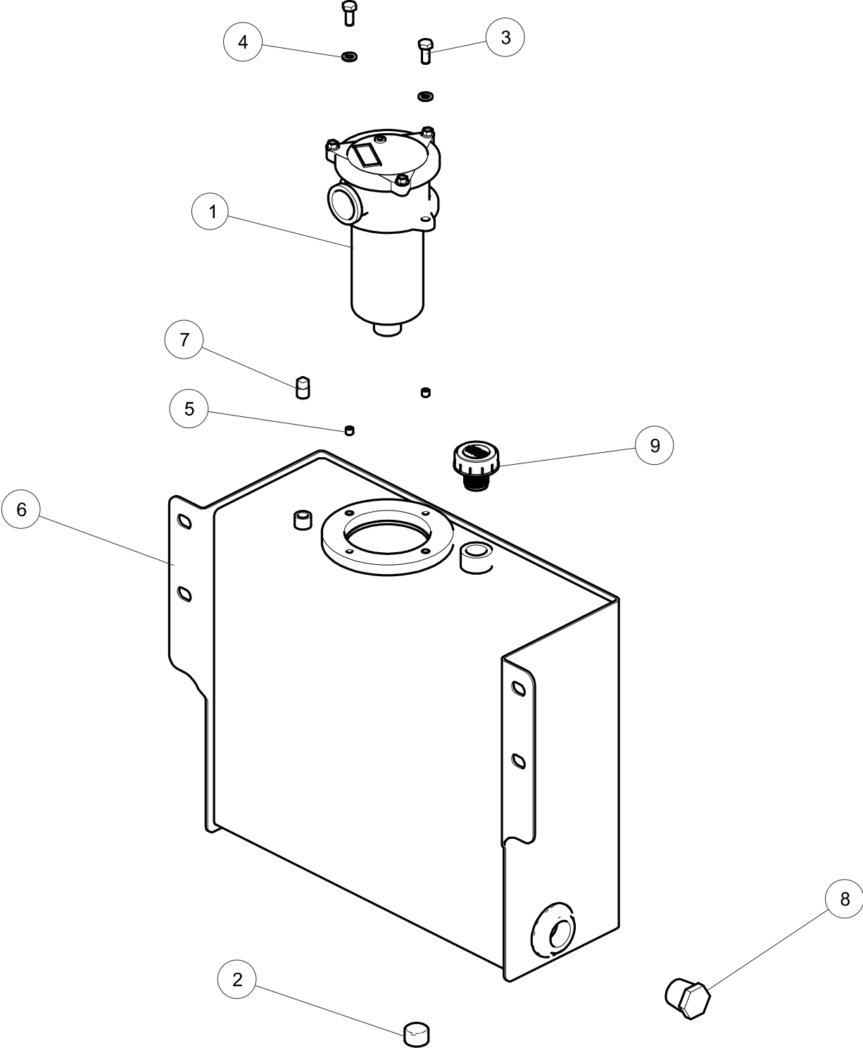
Figure 6. 812 Tank Assembly Figure
